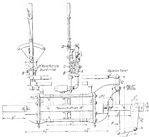
A Simple Power Reverse Gear
